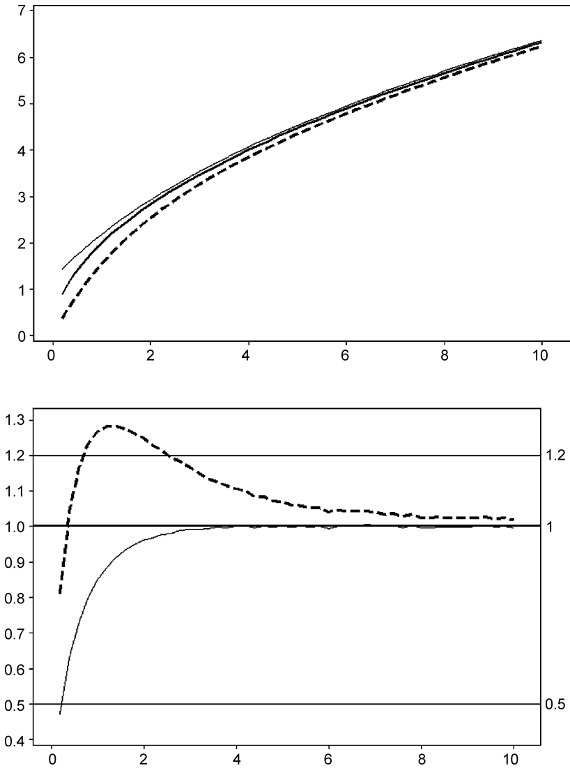
Figure 17.2 Let X \sim \text{Poisson}(\mu) . The graph of SD_\mu[\sqrt{4X}] versus \mu is shown in the bottom plot as a dashed line, and SD_\mu[\sqrt{4(X + 3/8)}] as a thin solid line. In the top plot are shown the target \sqrt{4\mu} versus \mu as a thick solid line, and the expected values of the two transformed statistics E_\mu[\sqrt{4X}] and the Anscombe vst E_\mu[\sqrt{4(X + 3/8)}] introduced in Section 17.3.3 versus \mu as thick dashed and thin solid lines, respectively. For n observations, one can replace X by n\bar{X}_n and \mu by n\mu on the horizontal axis. Note that for n\mu \geq 5 , the Anscombe vst performs very well.
